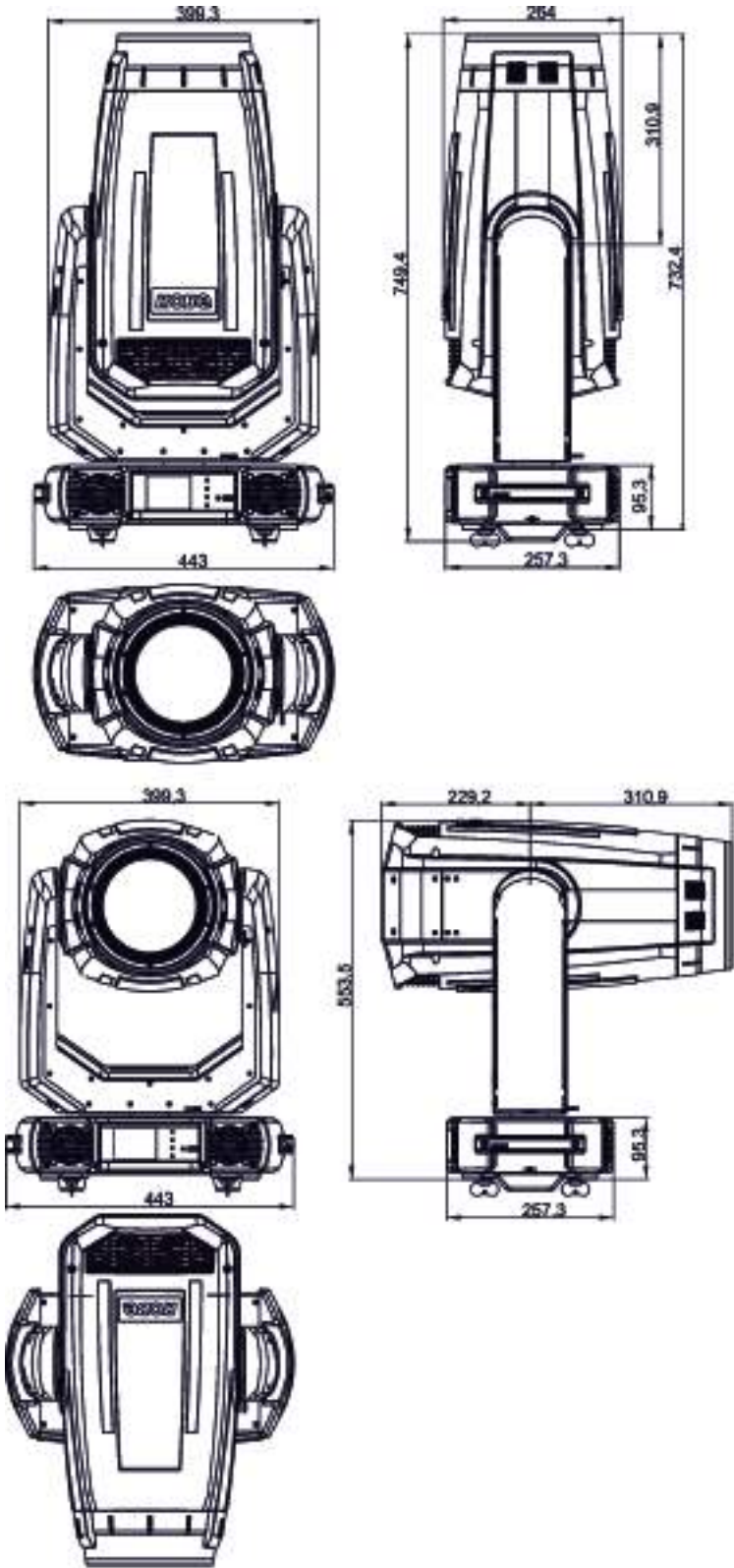
Dimensions (mm) Robin Esprite HCF
