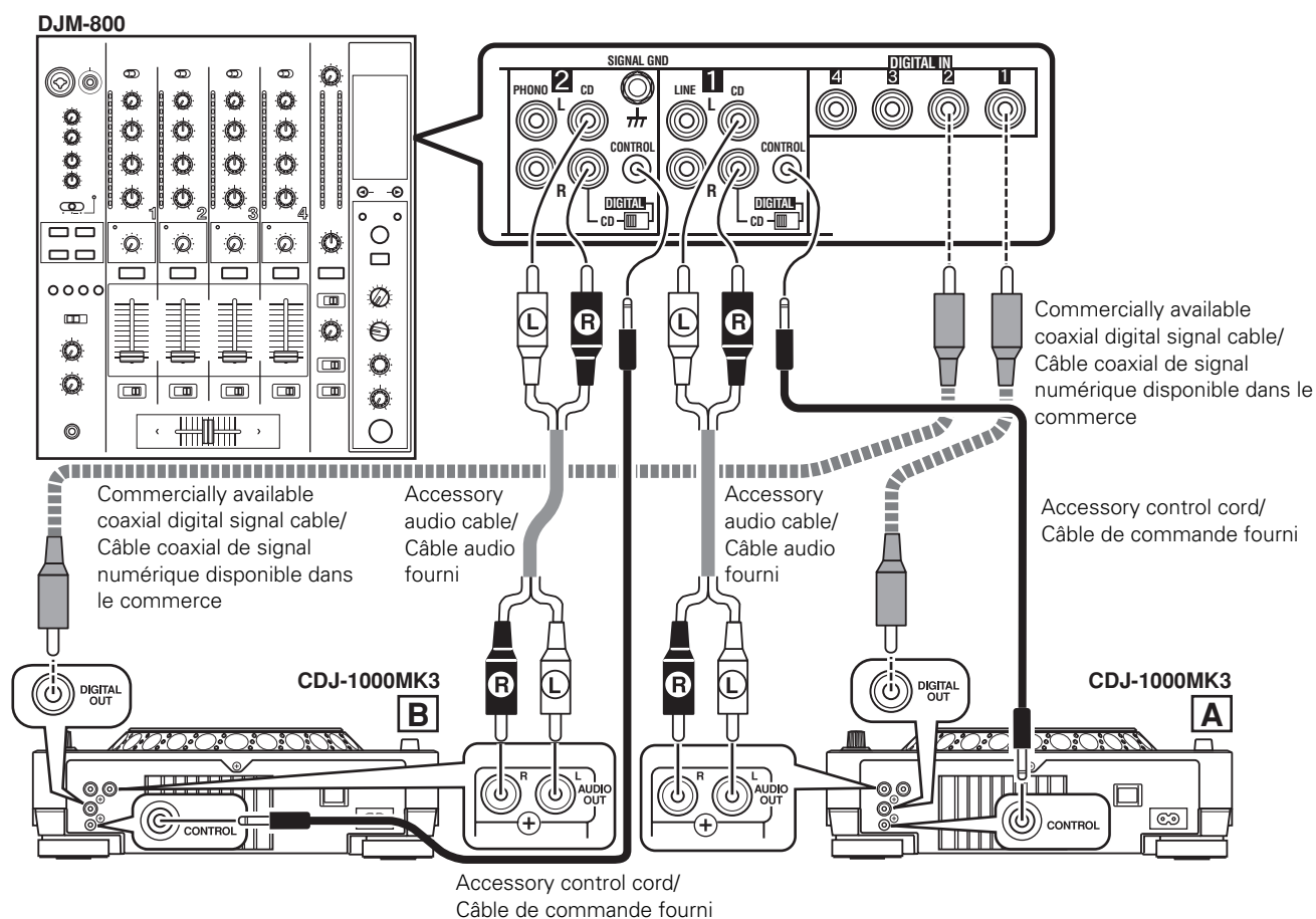
Connection example DJM-800:
