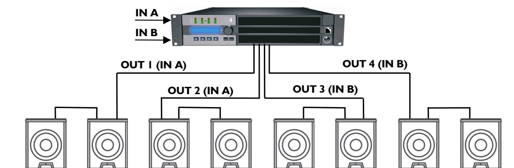
Figure 5: Eight 8XT enclosures connected to an LA4 / LA4X controller
