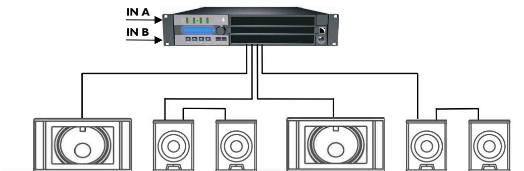
Figure 7: Four 8XT and two SB18 enclosures connected to an LA4 / LA4X controller
