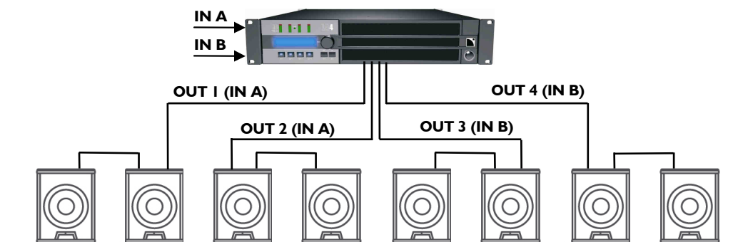
Figure 6: Eight 8XT enclosures connected to an LA4 / LA4X controller
