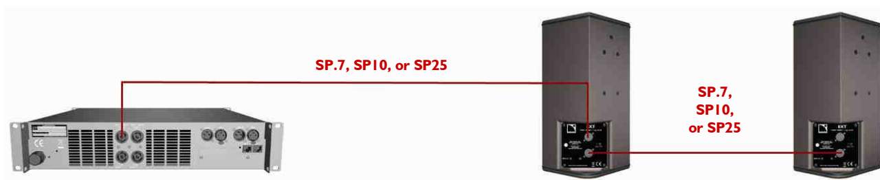
Figure 4: Connecting two 8XT in parallel to the LA4 / LA4X amp channel #1
