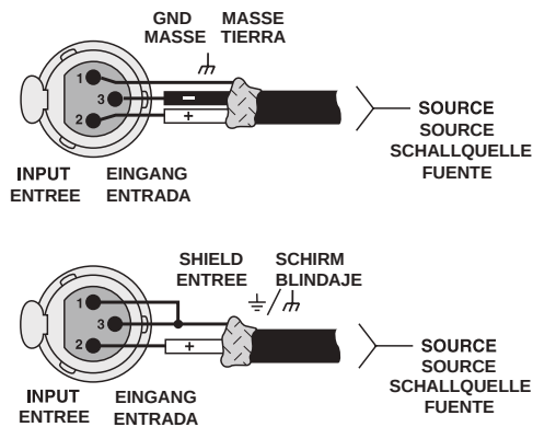
Figure 2.3 Input Connector XLR Wiring, Balanced (Top) and Unbalanced (Bottom)
