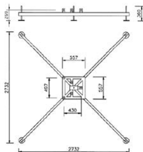
Type EMB ..... Embase
